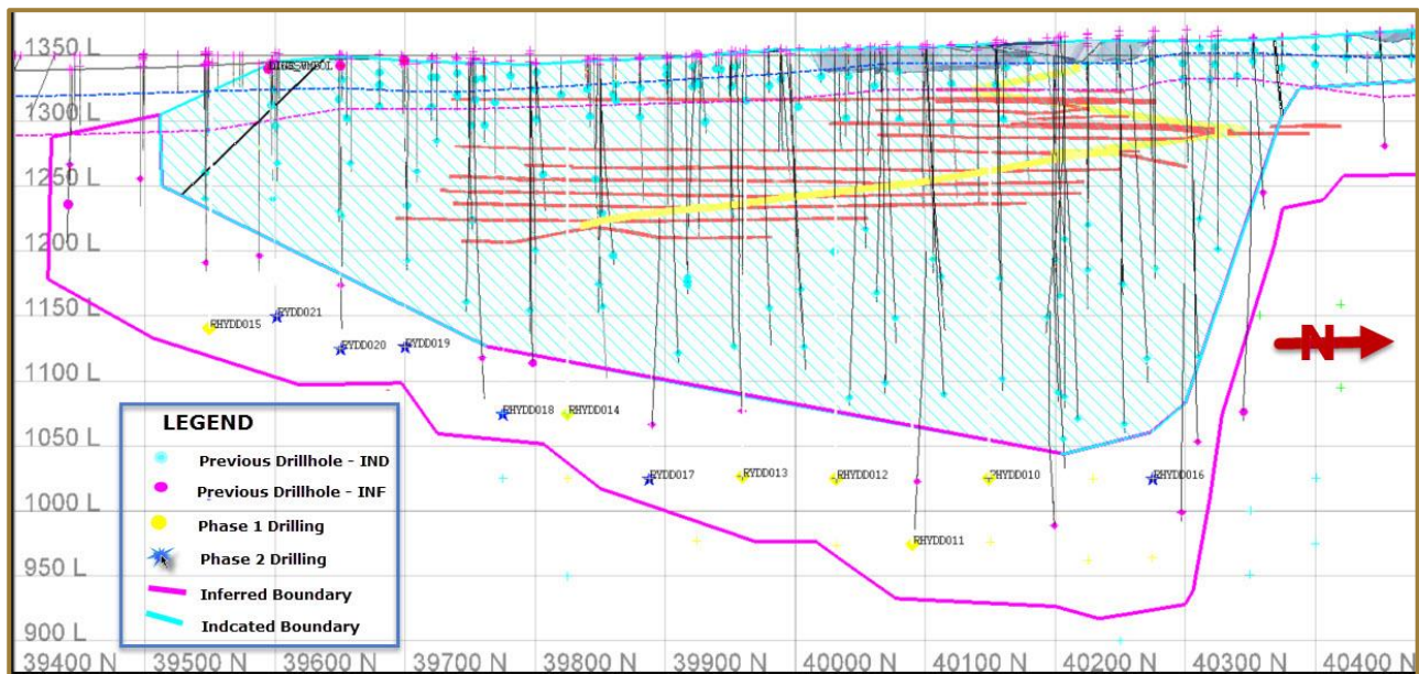
Figure 1 - "A" Shear long projection showing pierce points of proposed phase 2 drilling, proposed phase 1 drilling, previously drilled holes situated within Indicated and Inferred portions of the Mineral Resource and historic underground mine infrastructure
